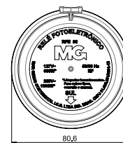
RFE-80 Top view
