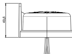
RFE-80 Side view
